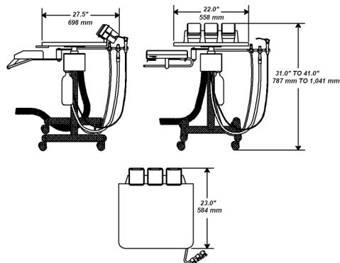
4081 and 4082 Dimensions
