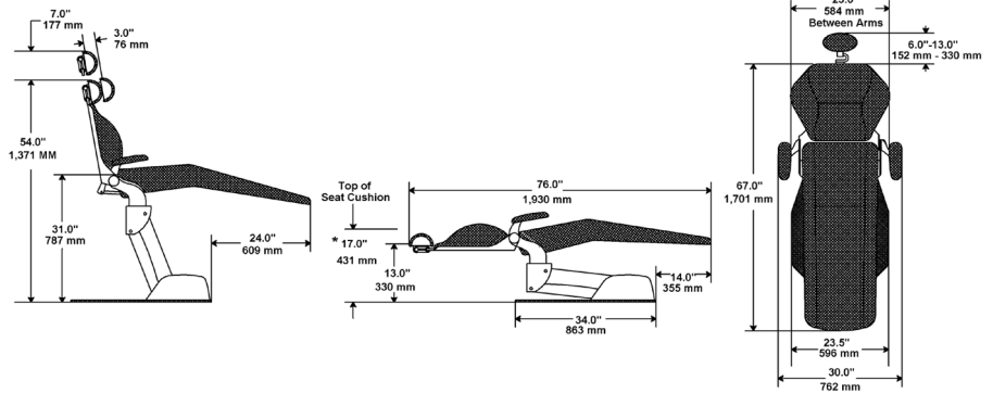
2001E Economy Asepsis Electromechanical Patient Chair
