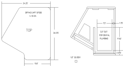
SP200 Standard Ortho Cart
