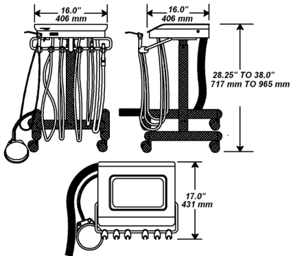
4085 Dimensions
